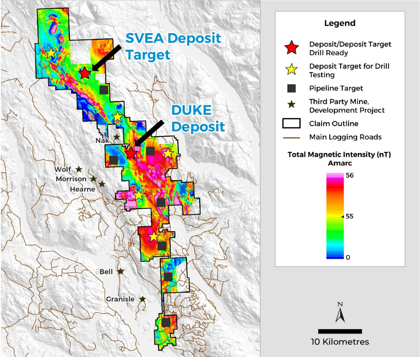
Figure 1: DUKE District – Comprehensive Exploration Surveys Have Delineated Multiple New Porphyry Cu-Au Targets
